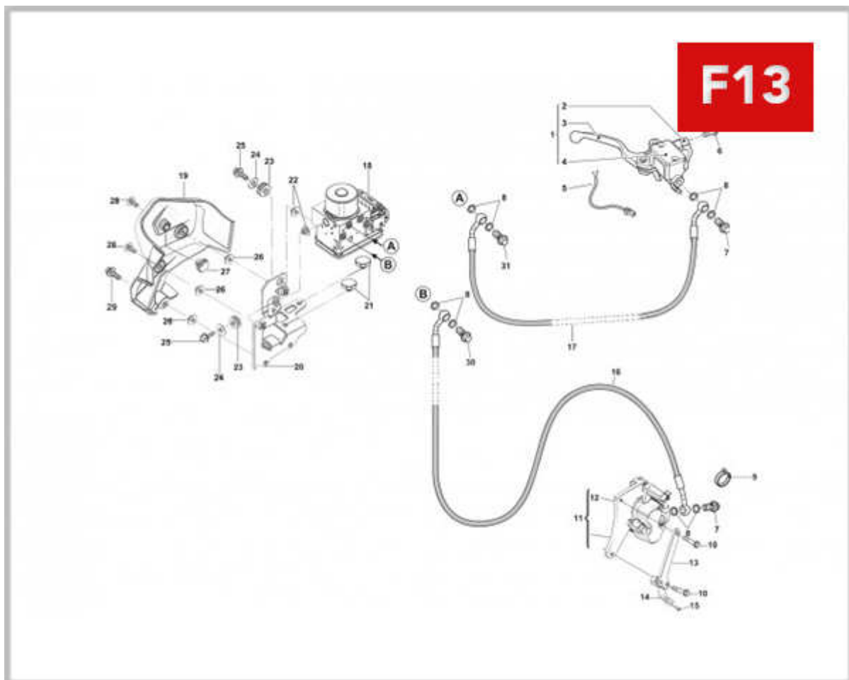
1 FA00A01289 FRONT LIQUID PRESSING PUMP
